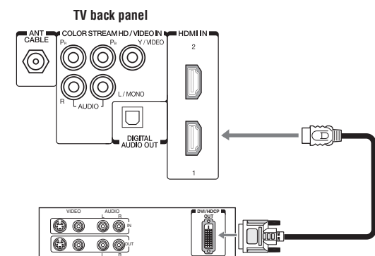
(Sample Illustration) DVI connections
